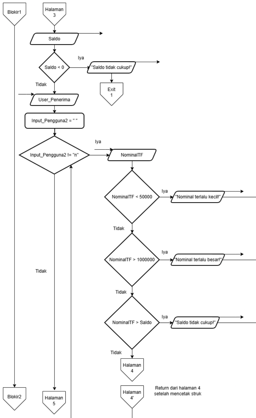
Gambar 1.3 Halaman 3 Flowchart
