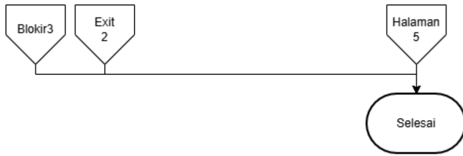
Gambar 1.5 Halaman 5 Flowchart
