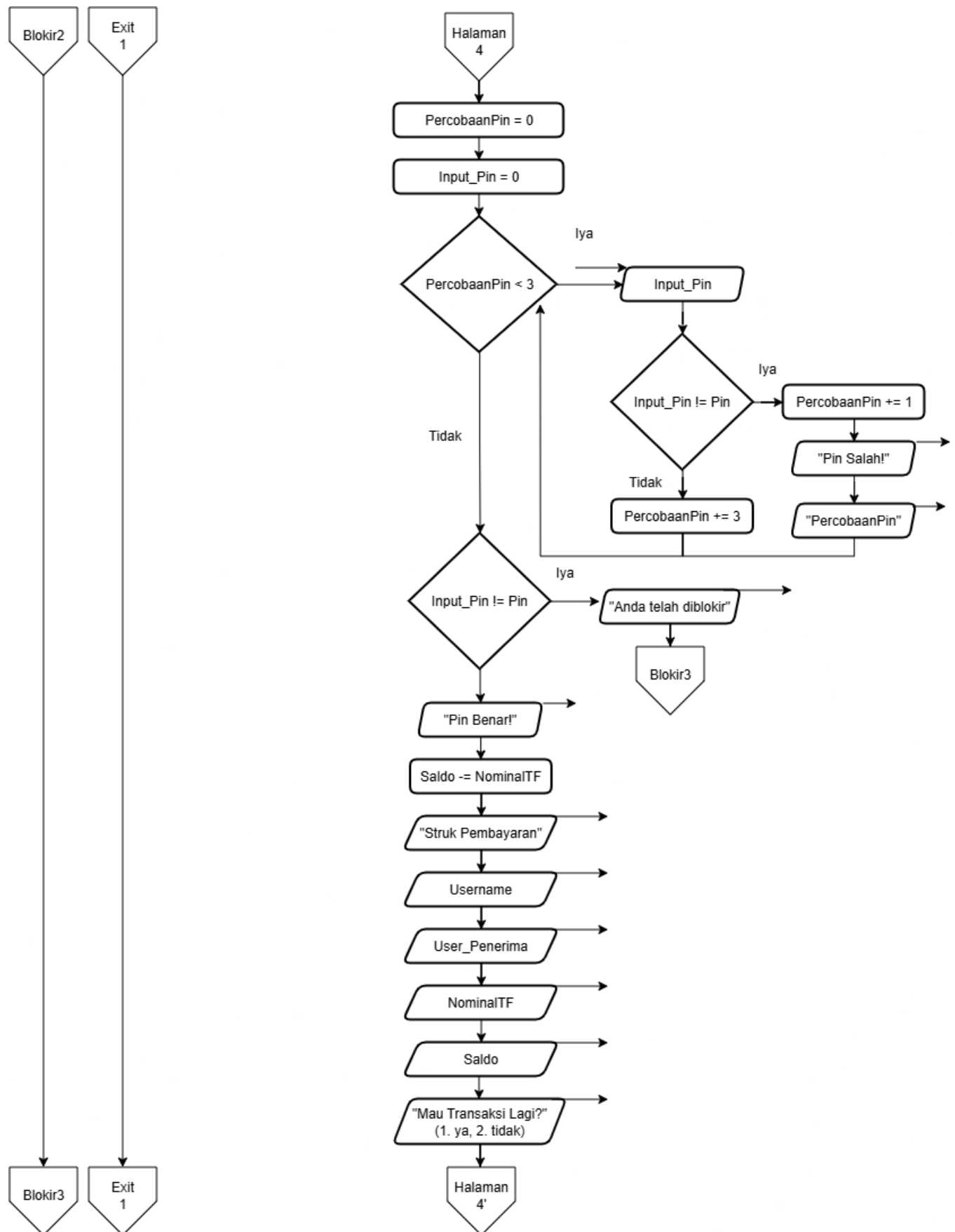
Gambar 1.4 Halaman 4 Flowchart
