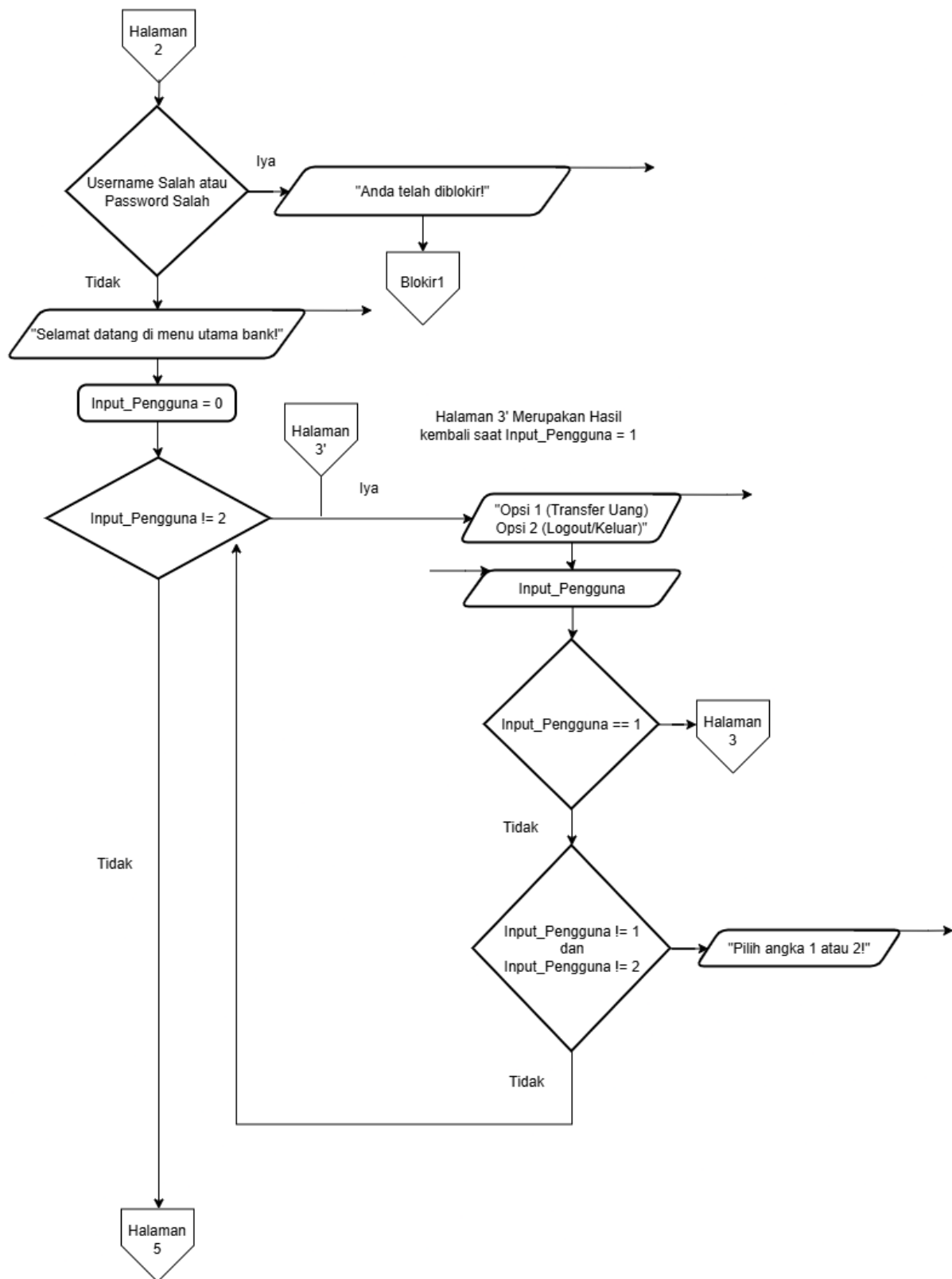
Gambar 1.2 Halaman 2 Flowchart
